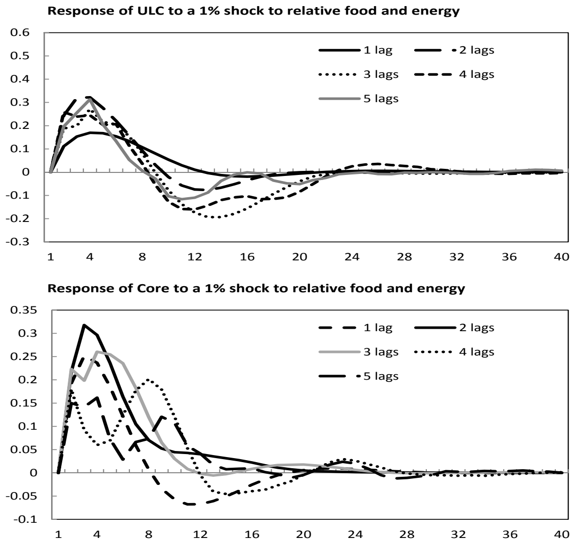
Figure 7: Sensitivity to lag length
