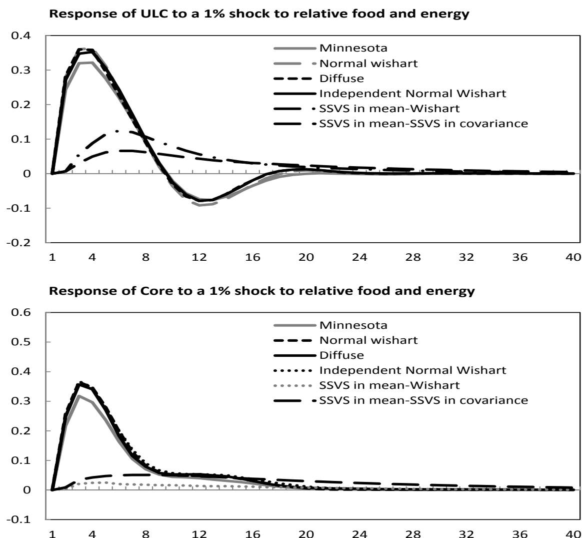
Figure 5: Sensitivity to prior selection
