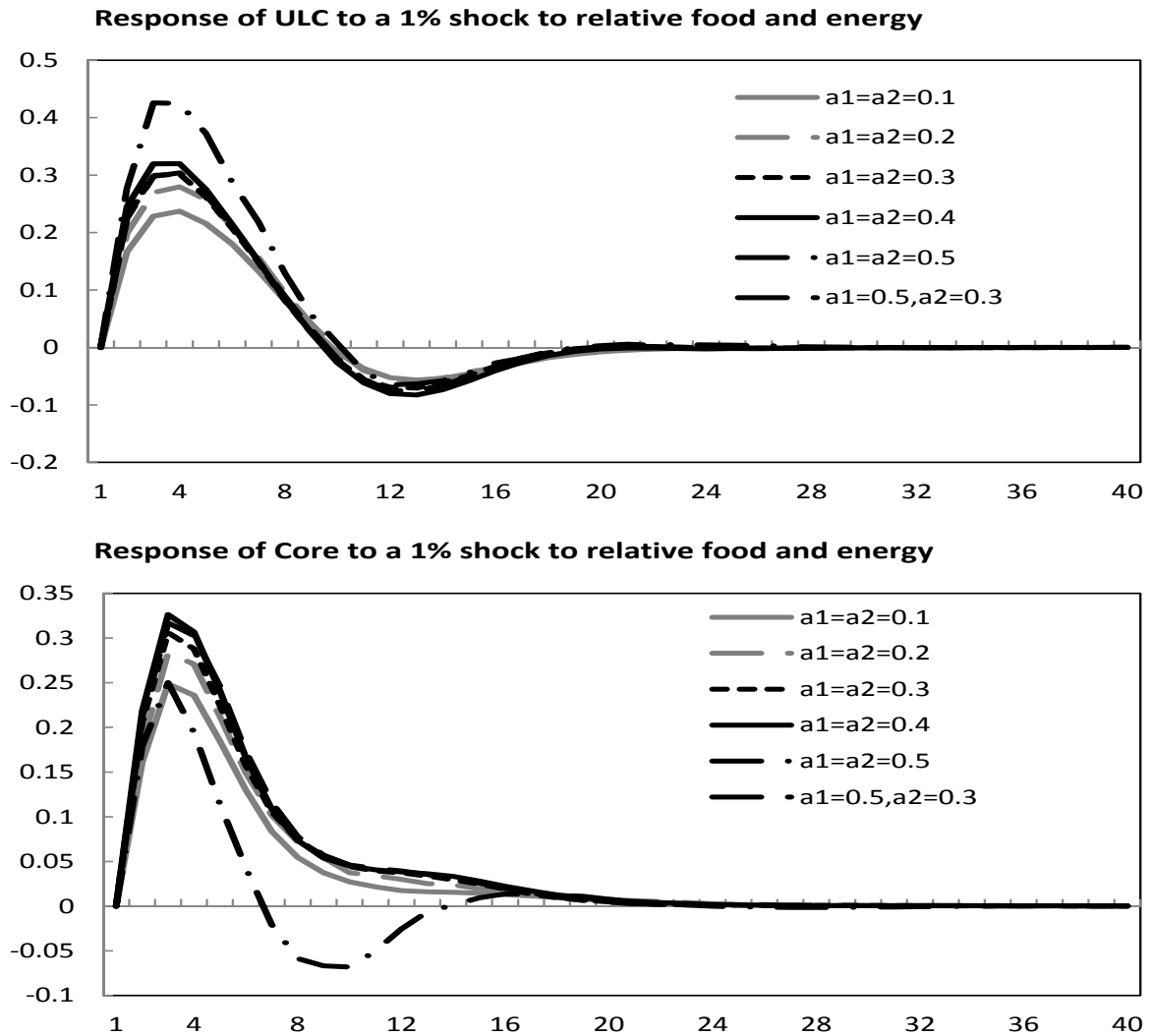
Figure 6: Sensitivity to prior hyperparameters
