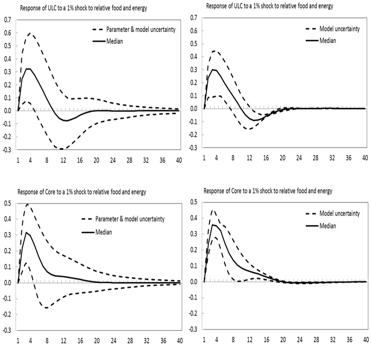
Figure 4: Model versus parameter uncertainty
