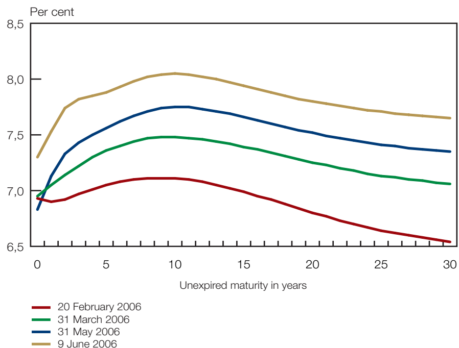
Yield curves
